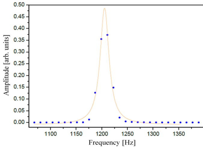
Fig. 5. Lorenz curve fit to the FFT-peak of the MEMS scanner decay curve after deflecting the scanner and turning off the drive voltage.
